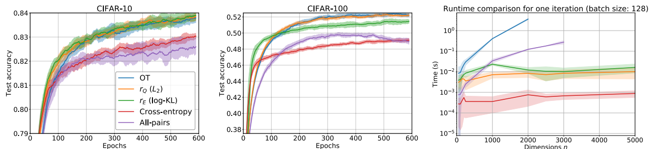
Figure 4. Left, center: Accuracy comparison on CIFAR-10, CIFAR-100 ( n = 10, n = 100 ). Right: Runtime comparison for one batch computation with backpropagation disabled. OT and All-pairs go out-of-memory starting from n = 2000 and n = 3000 , respectively. With backpropagation enabled, the runtimes are similar but OT and All-pairs go out-of-memory at n = 1000 and n = 2500 , respectively.
