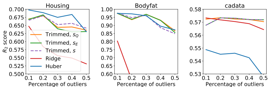
Figure 7. R_2 score (higher is better) averaged over 10 train-time splits for increasing percentage of outliers. Hyper-parameters are tuned by 5-fold cross-validation.
